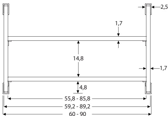
VISTA FRONTALE FRONT VIEW
