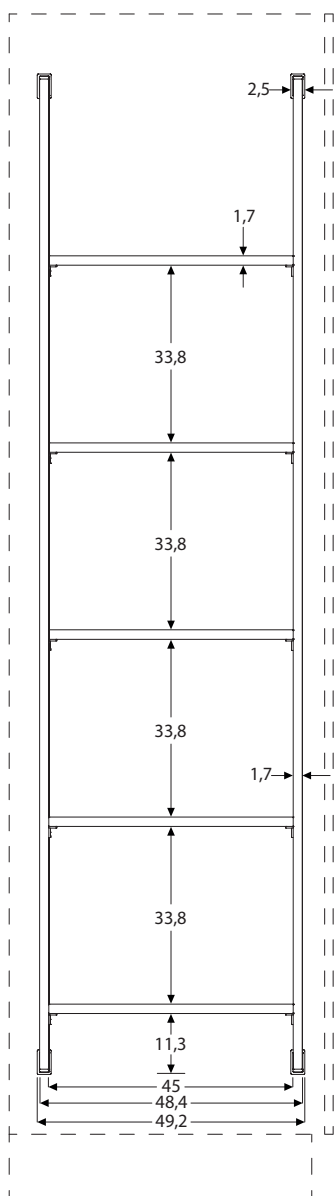
VISTA FRONTALE FRONT VIEW
